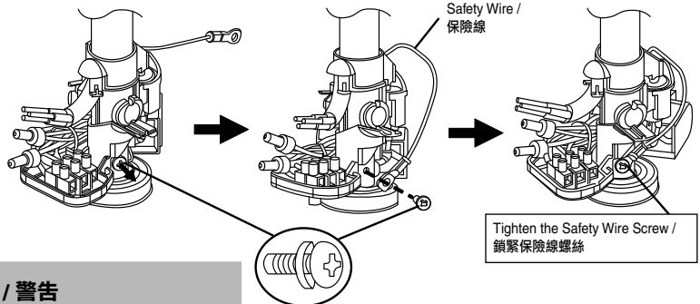
Safety Wire Screw (with washer) / 保險線螺絲 (配有墊圈)
